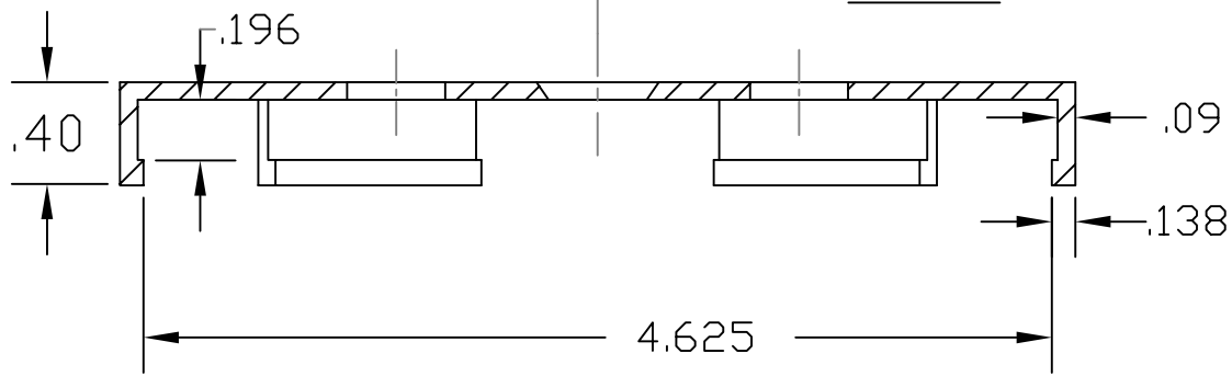
SECTION ELEVATION A-A
