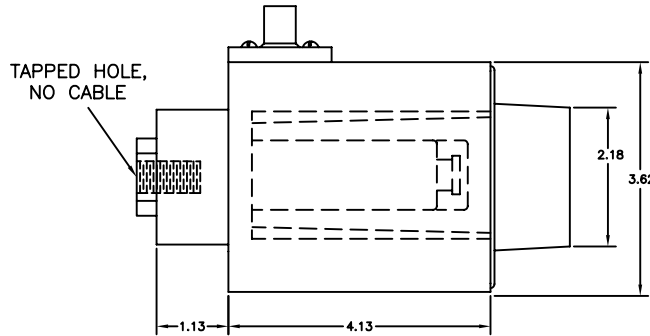
TAPPED HOLE BACK BLOCK
