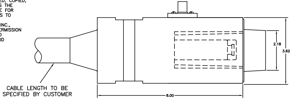
CABLE BACK BLOCK
