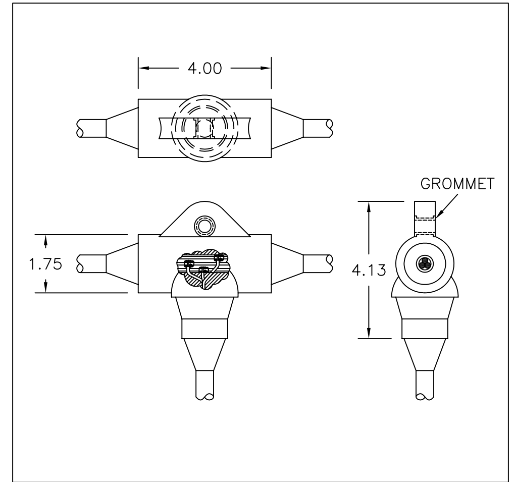
DETAIL 'A'
