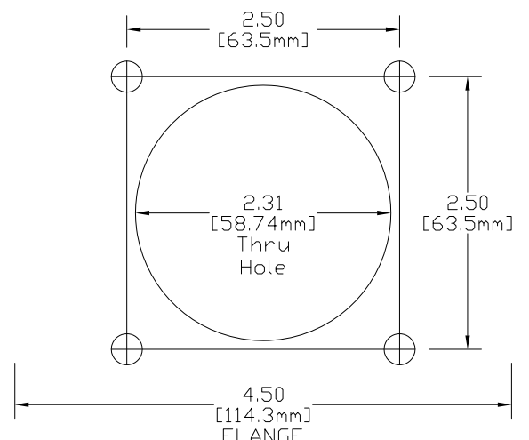
MOUNTING DIMENSIONS
