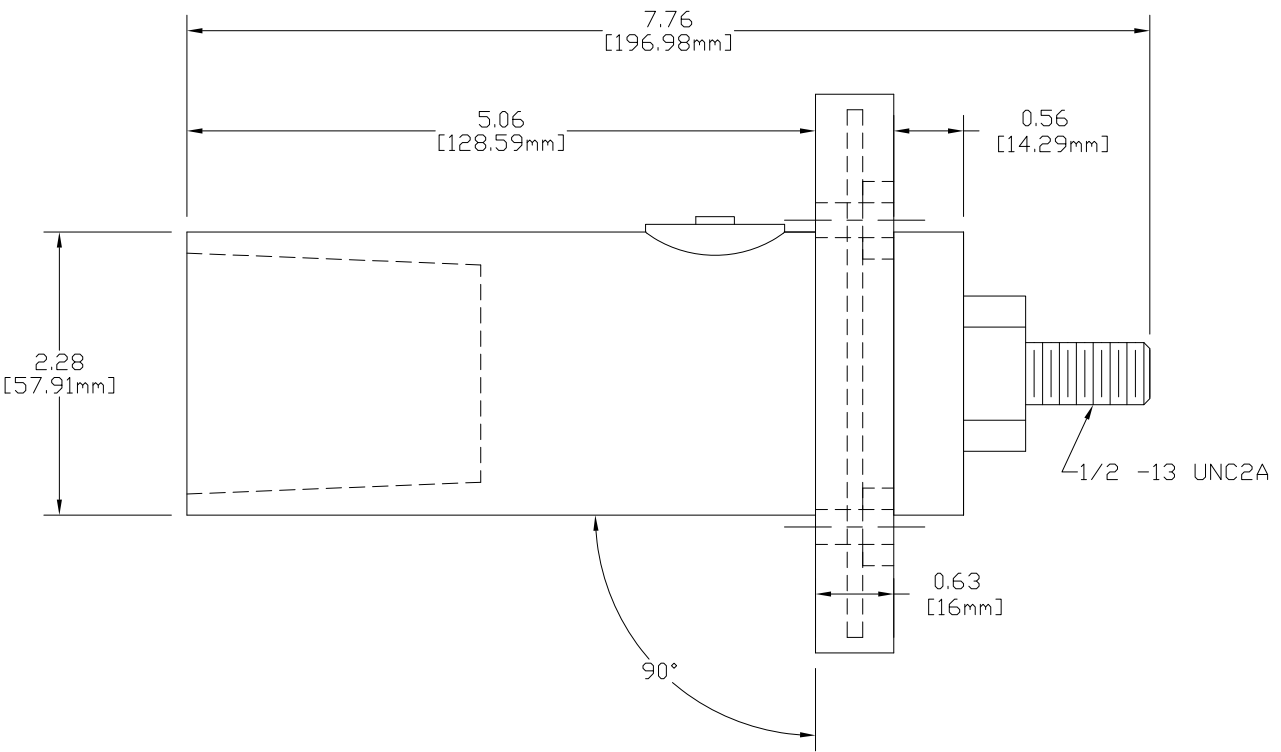
E1023 SERIES 90° POSITIVE LATCHING SERIES TAPERED NOSE - 23 SERIES MALE RECEPTACLE 350 - 750 MCM
