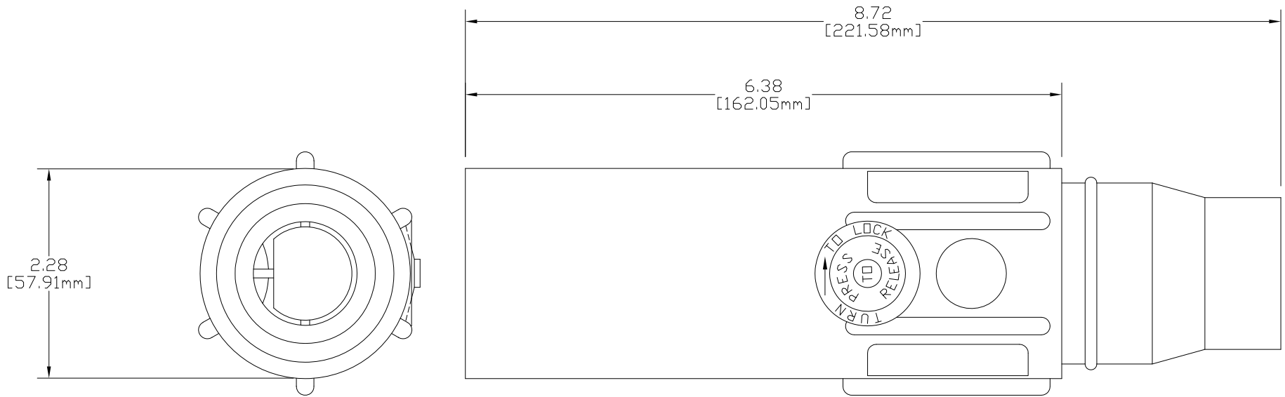
E1023 SERIES POSITIVE LATCHING "J" STYLE MALE TAPERED NOSE - 23 SERIES MALE CONNECTOR 350 - 500 MCM CABLE VULCANIZED
