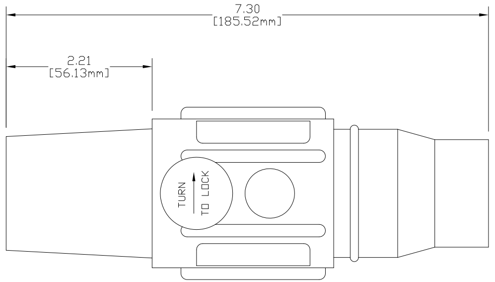
E1023 SERIES POSITIVE LATCHING "J" STYLE TAPERED NOSE - 23 SERIES FEMALE CONNECTOR 350 - 500 MCM CABLE VULCANIZED
