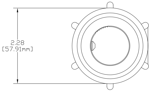
E1023 SERIES POSITIVE LATCHING "J" STYLE TAPERED NOSE - 23 SERIES FEMALE CONNECTOR 350 - 500 MCM CABLE VULCANIZED
