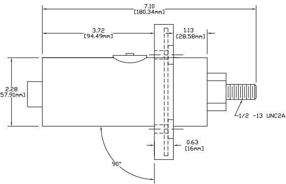
E1022 SERIES 90° POSITIVE LATCHING SERIES BALL NOSE - 22 SERIES MALE RECEPTACLE WITH UNLOCKING BUTTON 350 - 750 MCM
