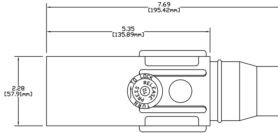
E1022 SERIES POSITIVE LATCHING SERIES BALL NOSE - 22 SERIES MALE CONNECTOR 350 - 500 MCM VULCANIZED
