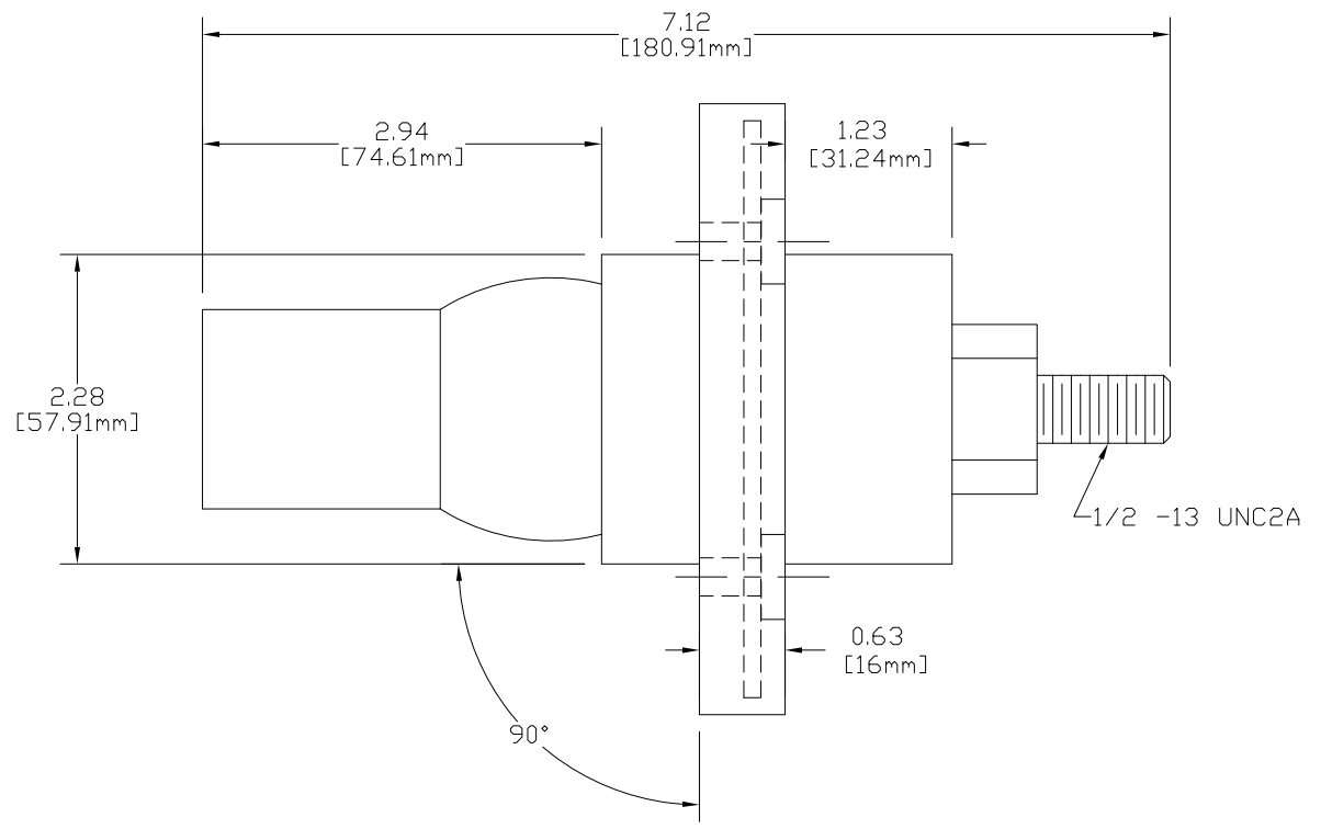
E1022 SERIES 90° POSITIVE LATCHING SERIES BALL NOSE - 22 SERIES FEMALE RECEPTACLE 350 - 750 MCM
