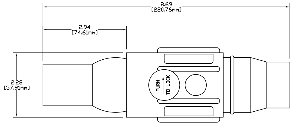
E1022 SERIES POSITIVE LATCHING SERIES BALL NOSE - 22 SERIES FEMALE CONNECTOR 350 - 500 MCM VULCANIZED
