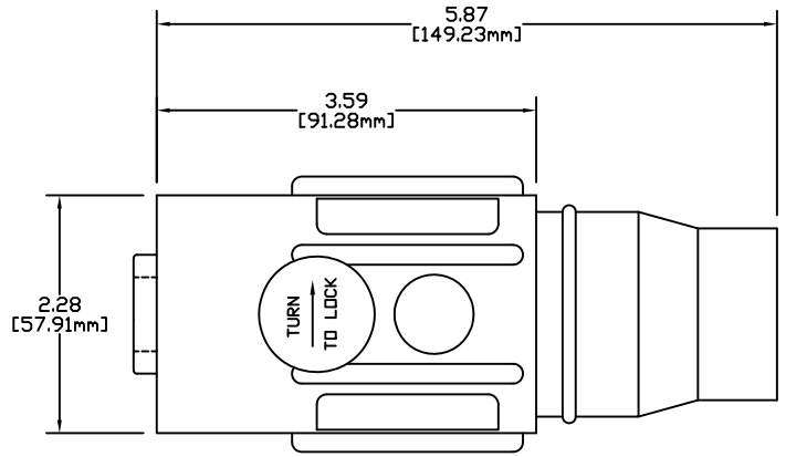
E1019 SERIES WELDING SERIES BALL NOSE - 19 SERIES MALE CONNECTOR 350 - 500 MCM VULCANIZED
