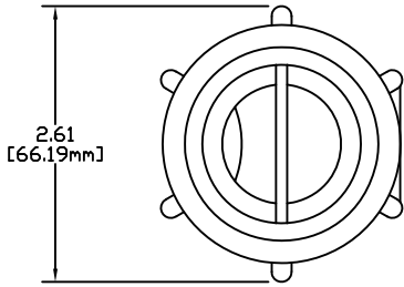
E1019 SERIES WELDING SERIES BALL NOSE - 19 SERIES MALE CONNECTOR 350 - 500 MCM VULCANIZED
