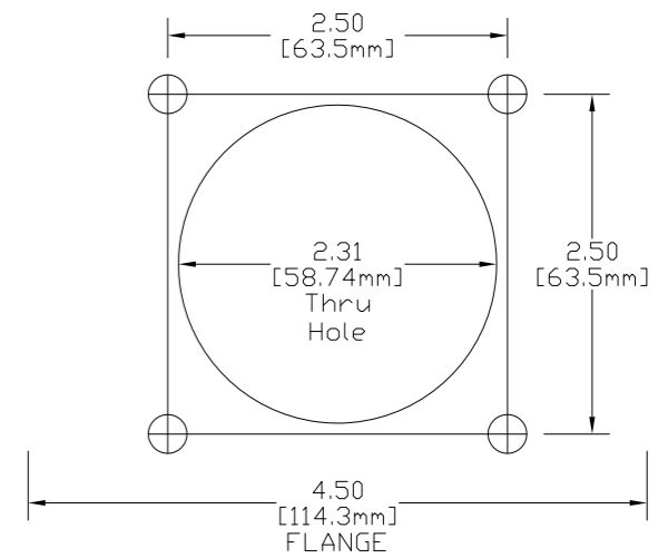
MOUNTING DIMENSIONS
