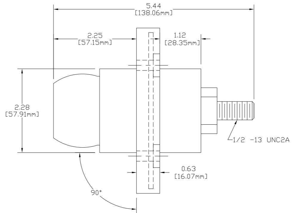
E1019 SERIES 90° WELDING SERIES BALL NOSE - 19 SERIES FEMALE RECEPTACLE 350 - 750 MCM
