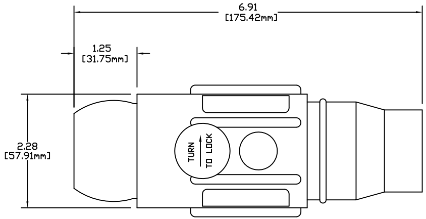
E1019 SERIES WELDING SERIES BALL NOSE - 19 SERIES FEMALE CONNECTOR 350 - 500 MCM VULCANIZED
