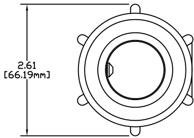
E1019 SERIES WELDING SERIES BALL NOSE - 19 SERIES FEMALE CONNECTOR 350 - 500 MCM VULCANIZED
