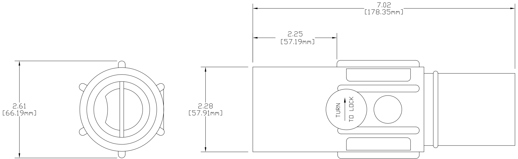
E1017 SERIES "J" SERIES TAPERED NOSE - 17 SERIES MALE CONNECTOR 750 - 800 MCM CABLE VULCANIZED
