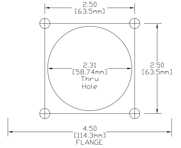
MOUNTING DIMENSIONS
