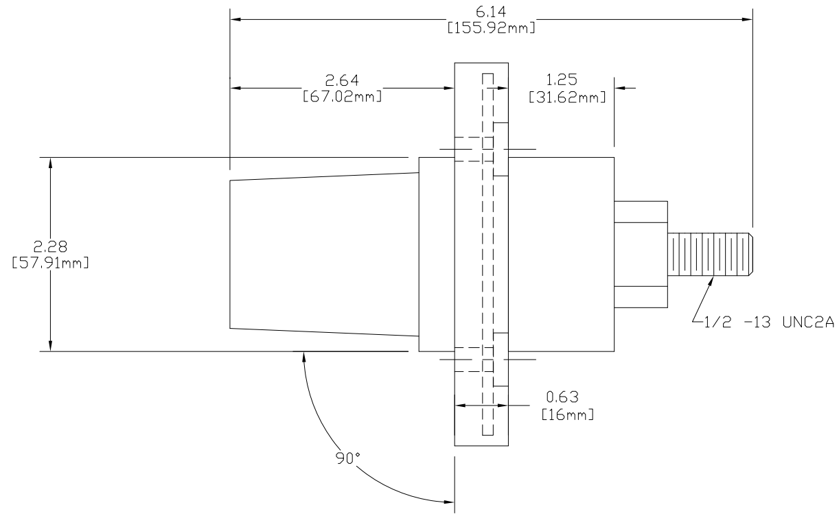
E1017 SERIES 90° "J" SERIES TAPERED NOSE - 17 SERIES FEMALE RECEPTACLE 350 - 750 MCM
