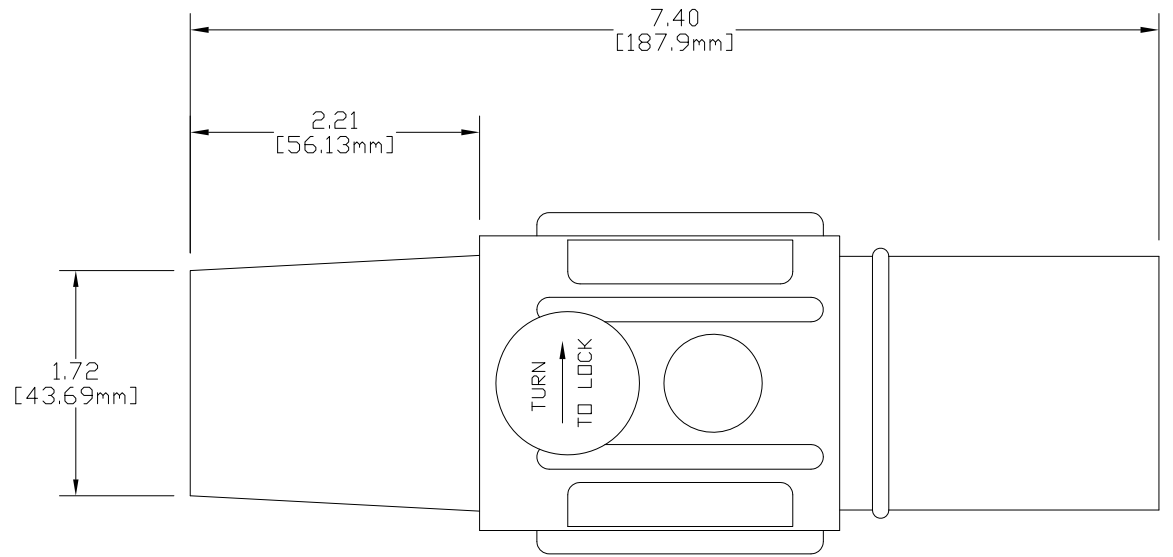
E1017 SERIES "J" SERIES TAPERED NOSE - 17 SERIES FEMALE CONNECTOR 750 - 800 MCM CABLE VULCANIZED
