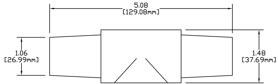
E1016 SERIES "J" SERIES 3 WAY LAY-DOWN "T" CONNECTOR - 16 SERIES DOUBLE FEMALE #2 - 4/0 CABLE
