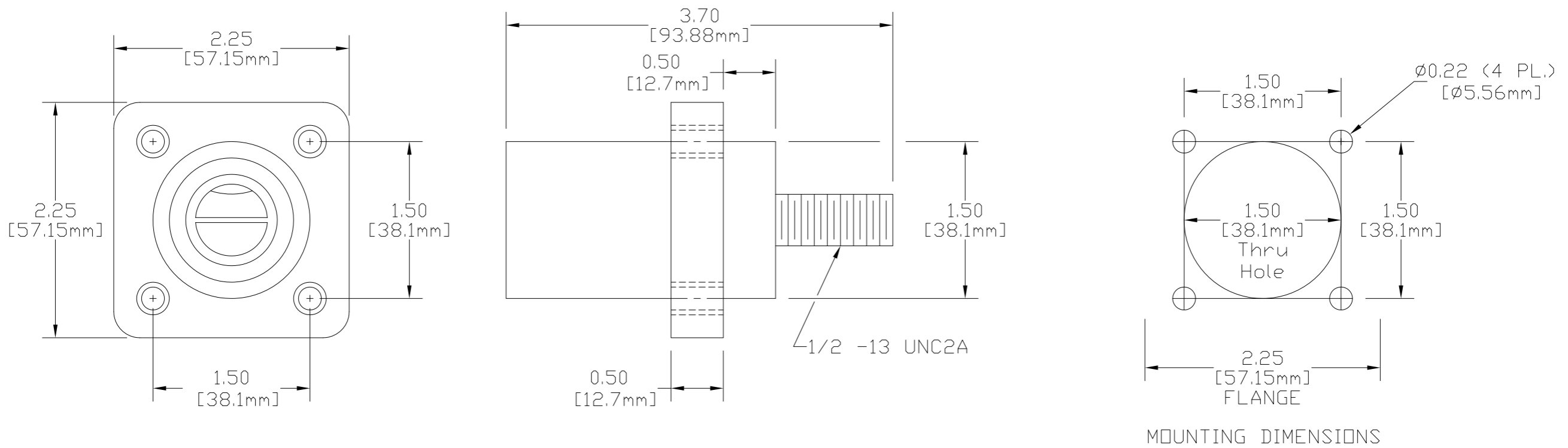
E1016 SERIES "J" SERIES THREADED STUD PANEL MOUNTS - 16 SERIES MALE RECEPTACLE #2 - 4/0 CABLE
