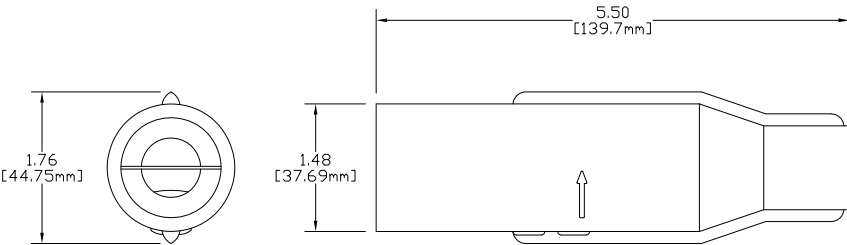
E1016 SERIES "J" SERIES TAPERED NOSE - 16 SERIES MALE CONNECTOR 1/0 - 2/0 CABLE VULCANIZED
