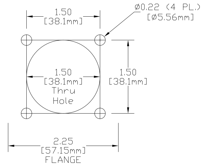
MOUNTING DIMENSIONS
