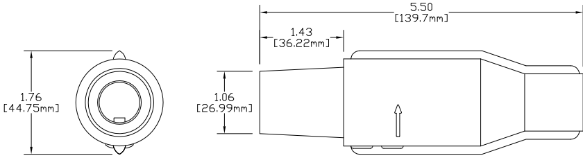
E1016 SERIES "J" SERIES TAPERED NOSE - 16 SERIES FEMALE CONNECTOR 1/0 - 2/0 CABLE VULCANIZED
