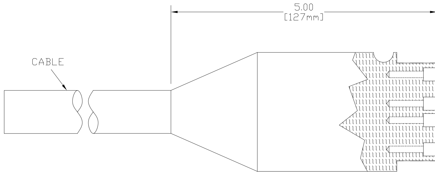
8FP10 FEMALE CONNECTOR
