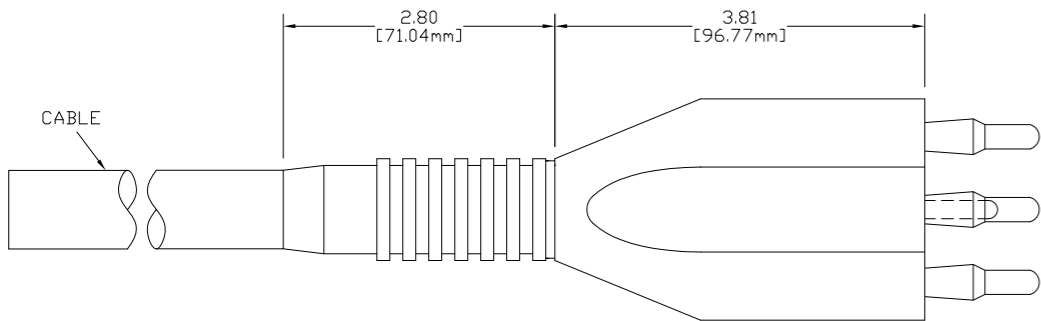
4M20 MALE CONNECTOR
