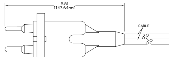
2MR30POL MALE CONNECTOR
