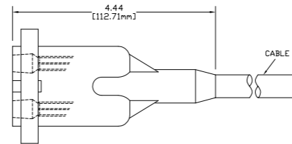
2FR18POL FEMALE CONNECTOR
