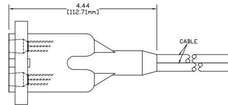
2FR30POL FEMALE CONNECTOR
