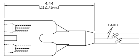
2F30POL FEMALE CONNECTOR
