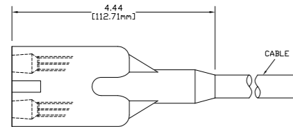
2F18POL FEMALE CONNECTOR
