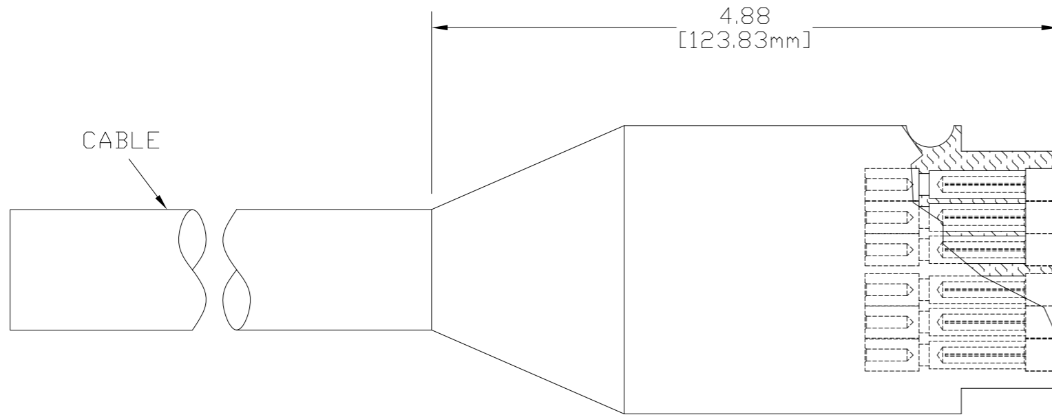
16FP7 FEMALE CONNECTOR
