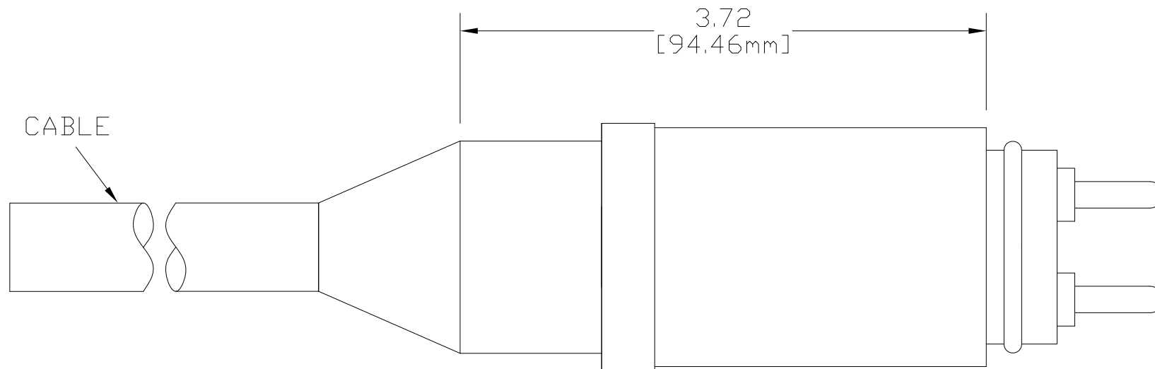
15MP3 MALE CONNECTOR
