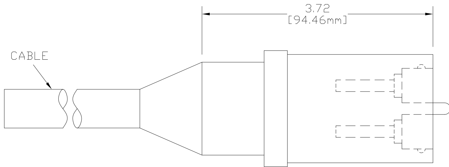
15FP3 FEMALE CONNECTOR
